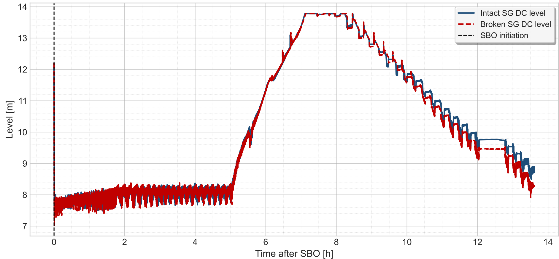
Base Case - Steam Generator DC Levels
